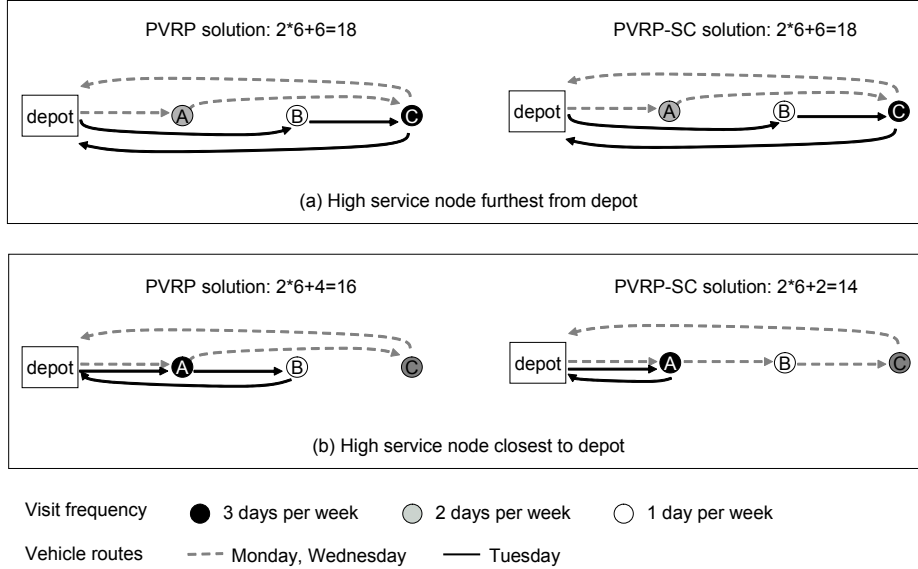
Figure 6: Impact of node distribution on routing efficiency due to service choice
