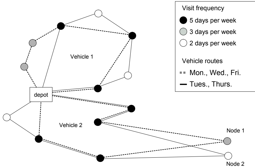
Figure 1: Period Vehicle Routing Problem
